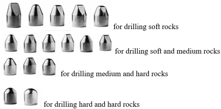
Figure 3. Carbide teeth
